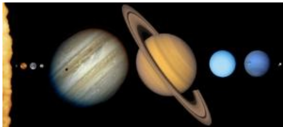
The Solar System
